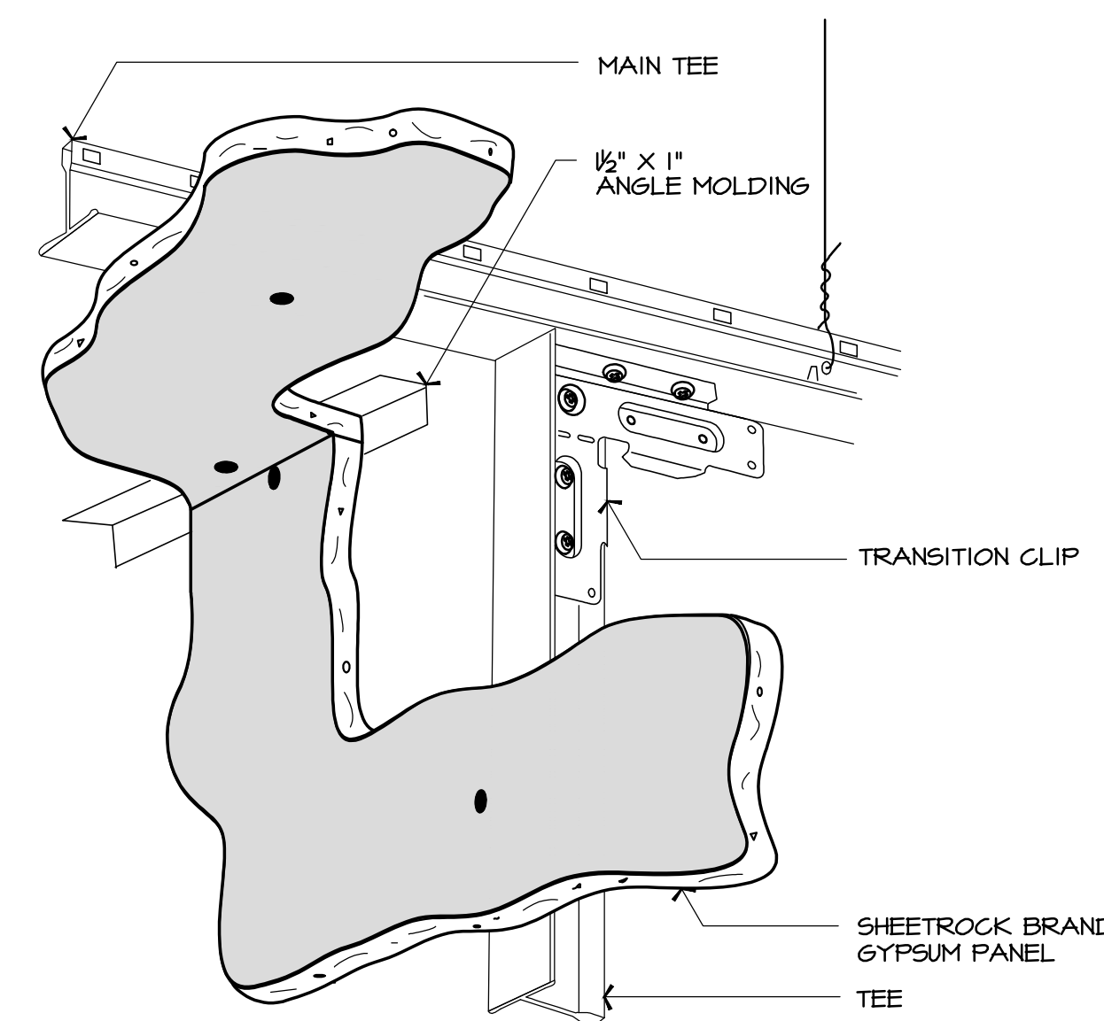
3 CORNER WITH FIELD CUT TEE CLG-CORNER FIELD CUT TEES.DWG SCALE: N.T.S.
