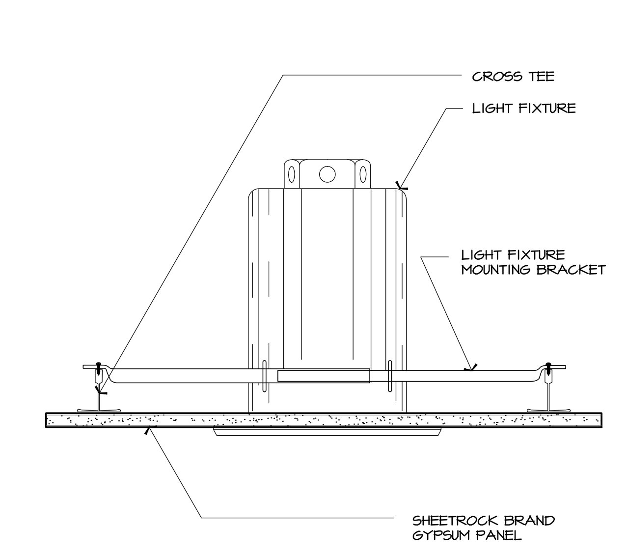
6 RECESSED LIGHT FIXTURE CLG-RECESSED-LIGHT.DWG SCALE: N.T.S.
