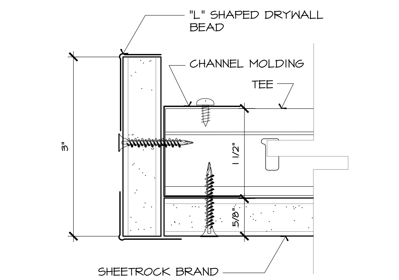
11 DETAIL @ GYP. BD. EDGE CLG-DETAIL-GYPEDGE.DWG SCALE: N.T.S.
