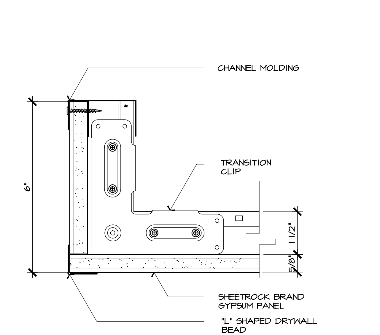
12 DETAIL @ TRANSITION DETAIL CLG-DETAIL-TRANSITION.DWG SCALE: N.T.S.
