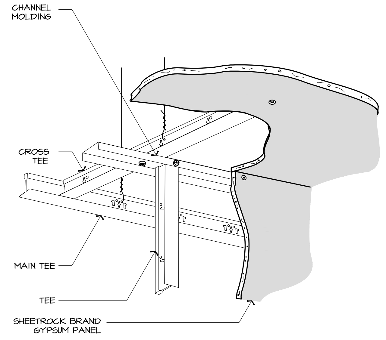
4 INSIDE CORNER WITH CHANNEL CLG-CORNER WITH CHANNEL MOLDING.DWG SCALE: N.T.S.
