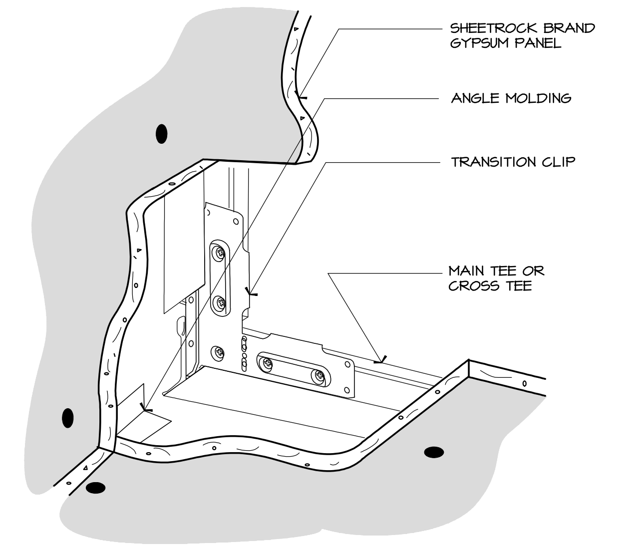
2 CORNER - TRANSITION CLIP CLG-CORNER USING TRANSITION.DWG SCALE: N.T.S.
