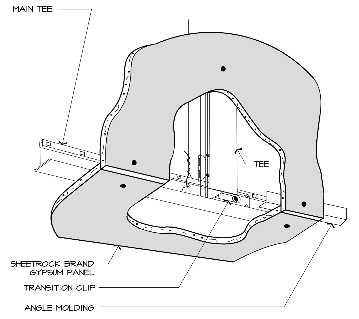
1 OUTSIDE CORNER DETAIL CLG-CORNER WITH MAIN TEES.DWG SCALE: N.T.S.
